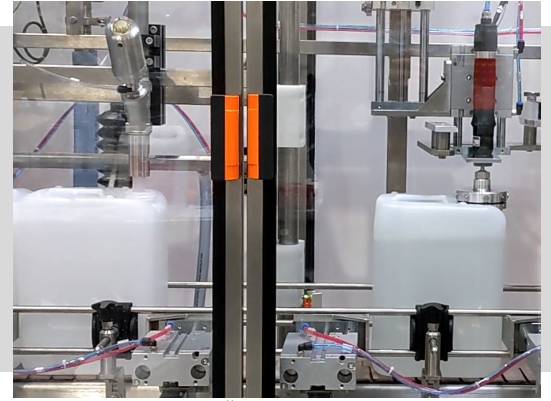
Filling capping
