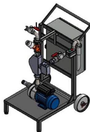
DN25 filling trolley
